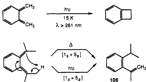
Scheme 40
