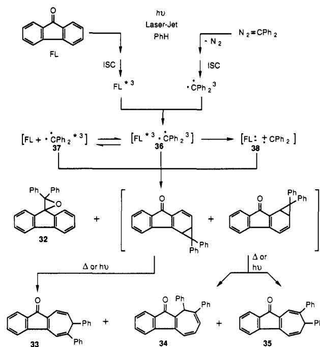
Scheme 12
