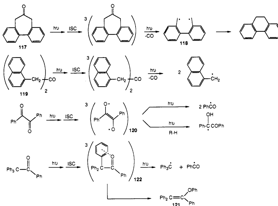
Scheme 45
