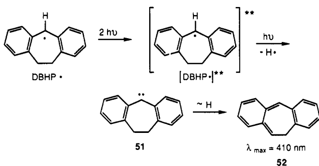
Scheme 17
