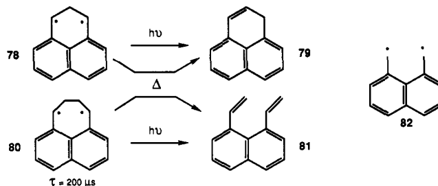
Scheme 28
