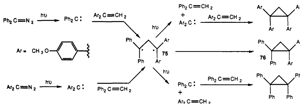
Scheme 28
