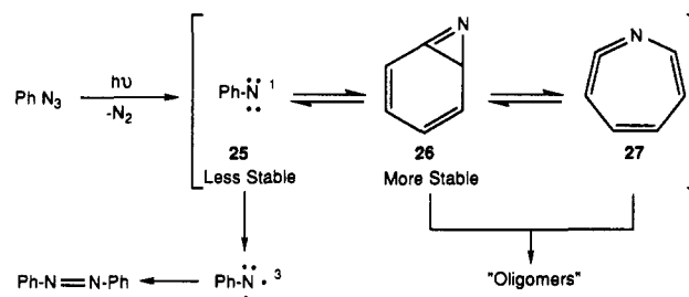
Scheme 10
