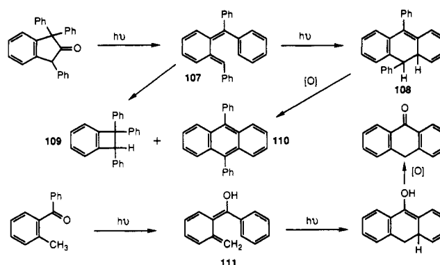
Scheme 41
