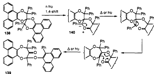
Scheme 52
