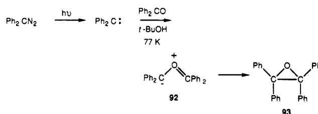
Scheme 34
