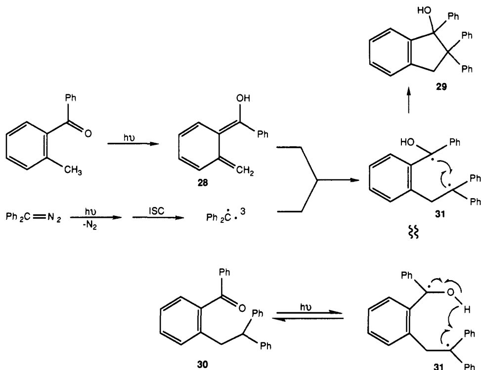
Scheme 12
