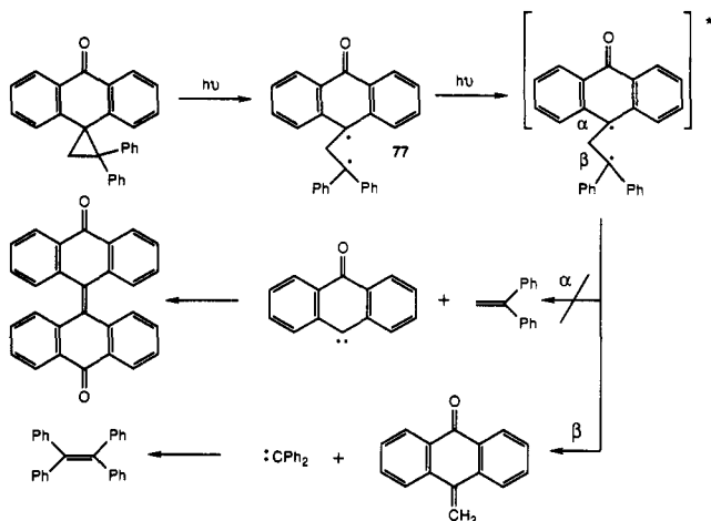
Scheme 27
