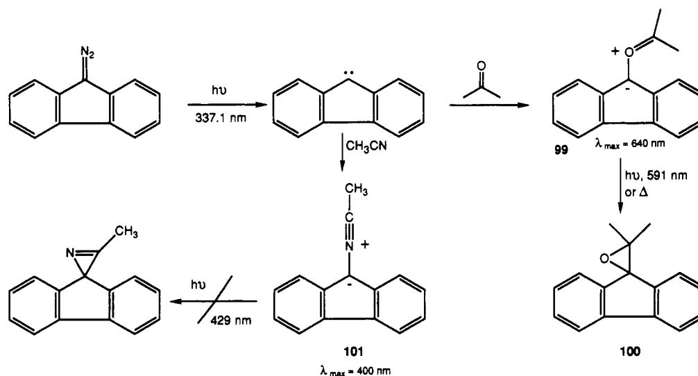
Scheme 41
