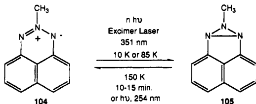
Scheme 40
